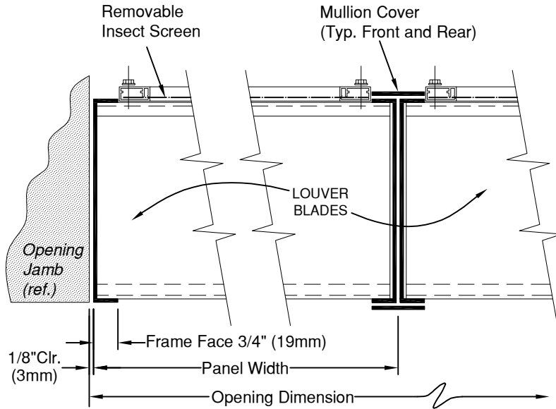
TYPICAL HORIZONTAL SECTION
