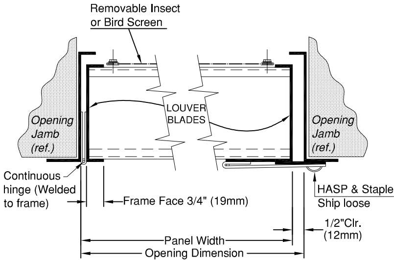
TYPICAL HORIZONTAL SECTION
