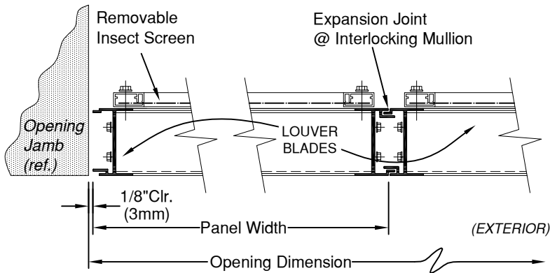
TYPICAL HORIZONTAL SECTION
