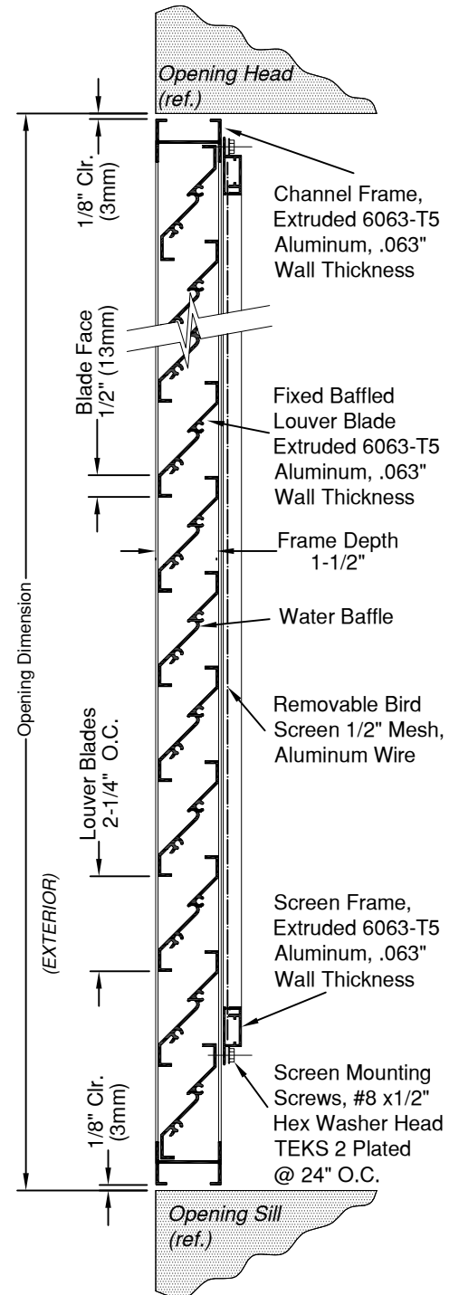
TYPICAL VERTICAL SECTION
