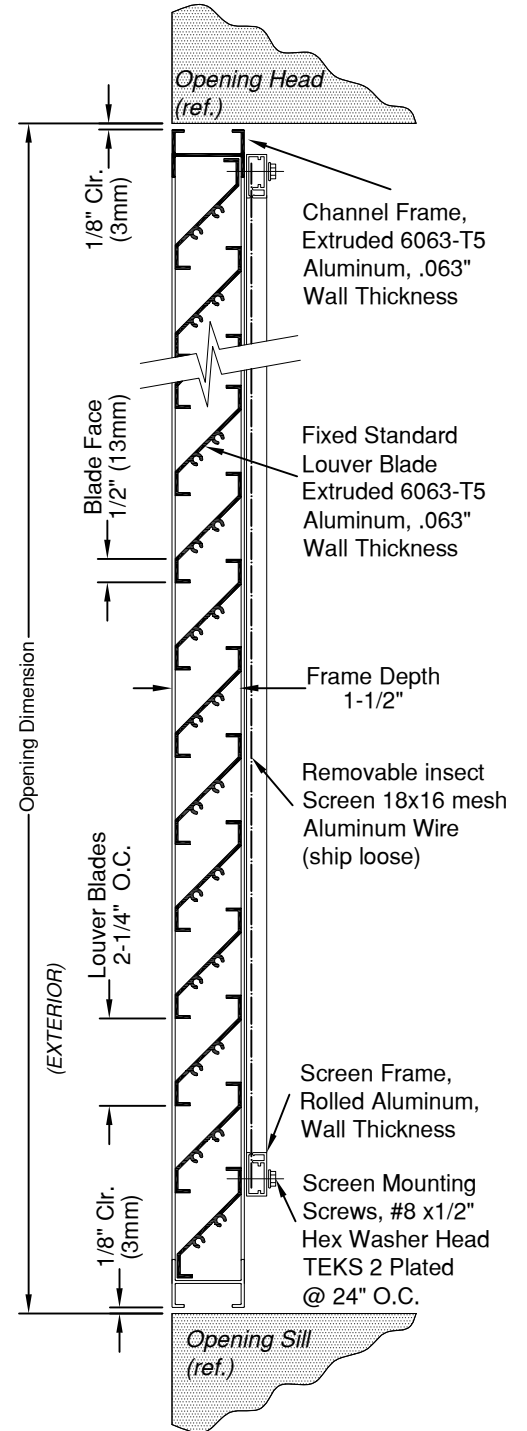
TYPICAL VERTICAL SECTION
