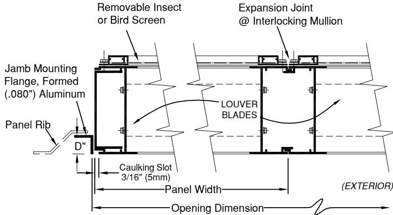
TYPICAL HORIZONTAL SECTION
