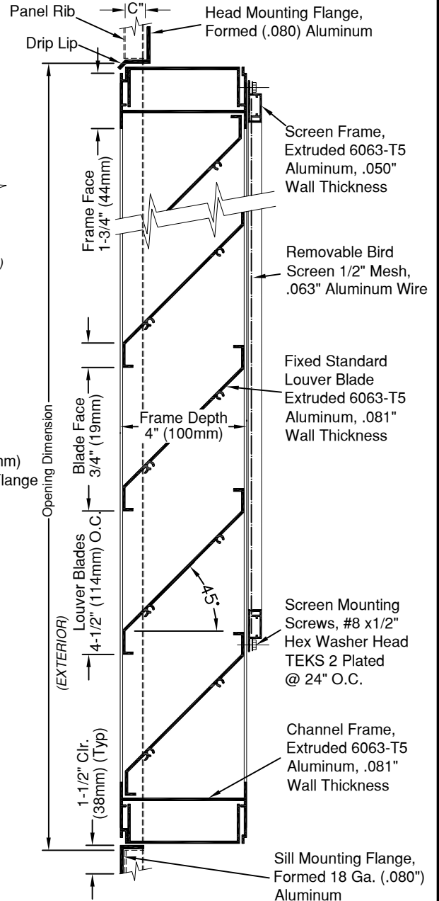
TYPICAL VERTICAL SECTION
