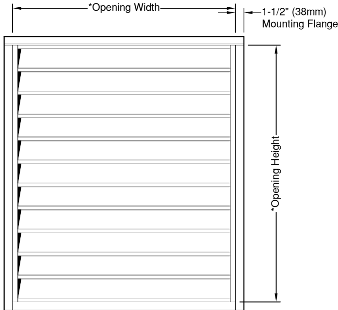
FRONT ELEVATION
