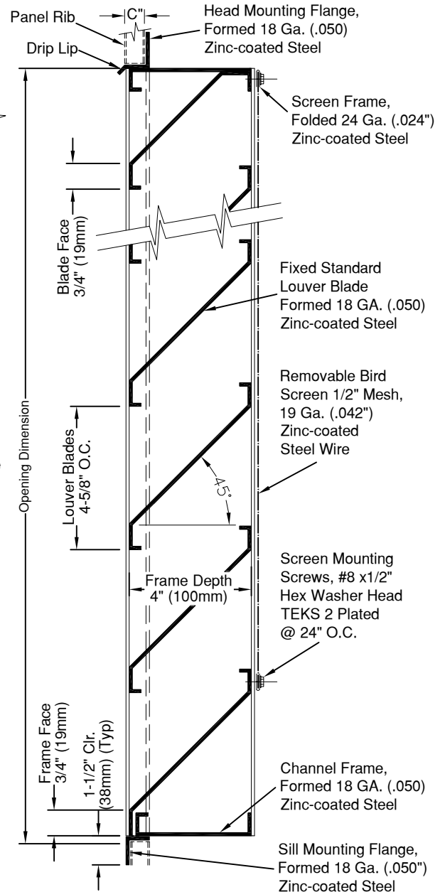
TYPICAL VERTICAL SECTION
